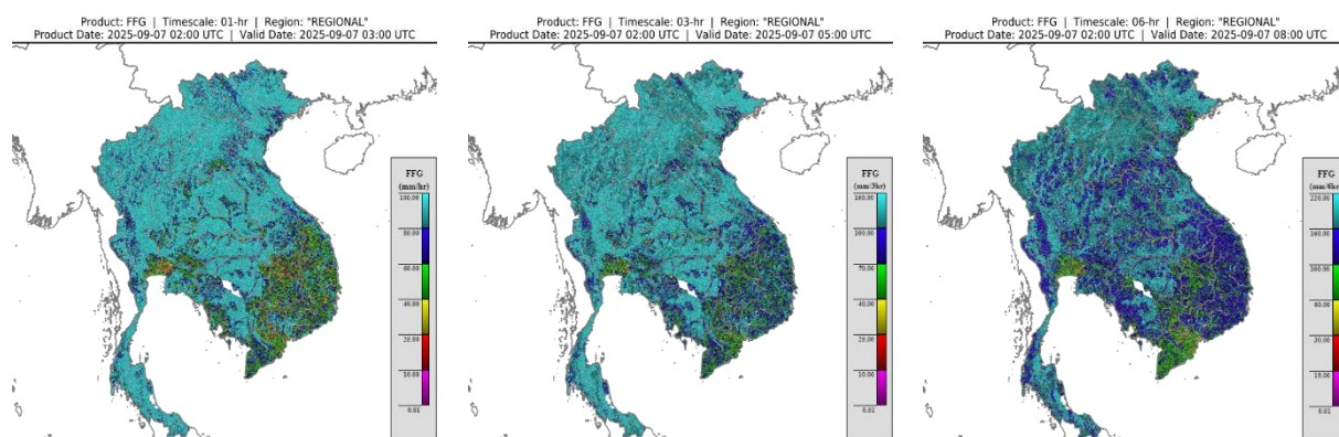
Figure 10. Flash Flood Guidance for the next 1-hr, 3-hr and 6-hr on 07 September
